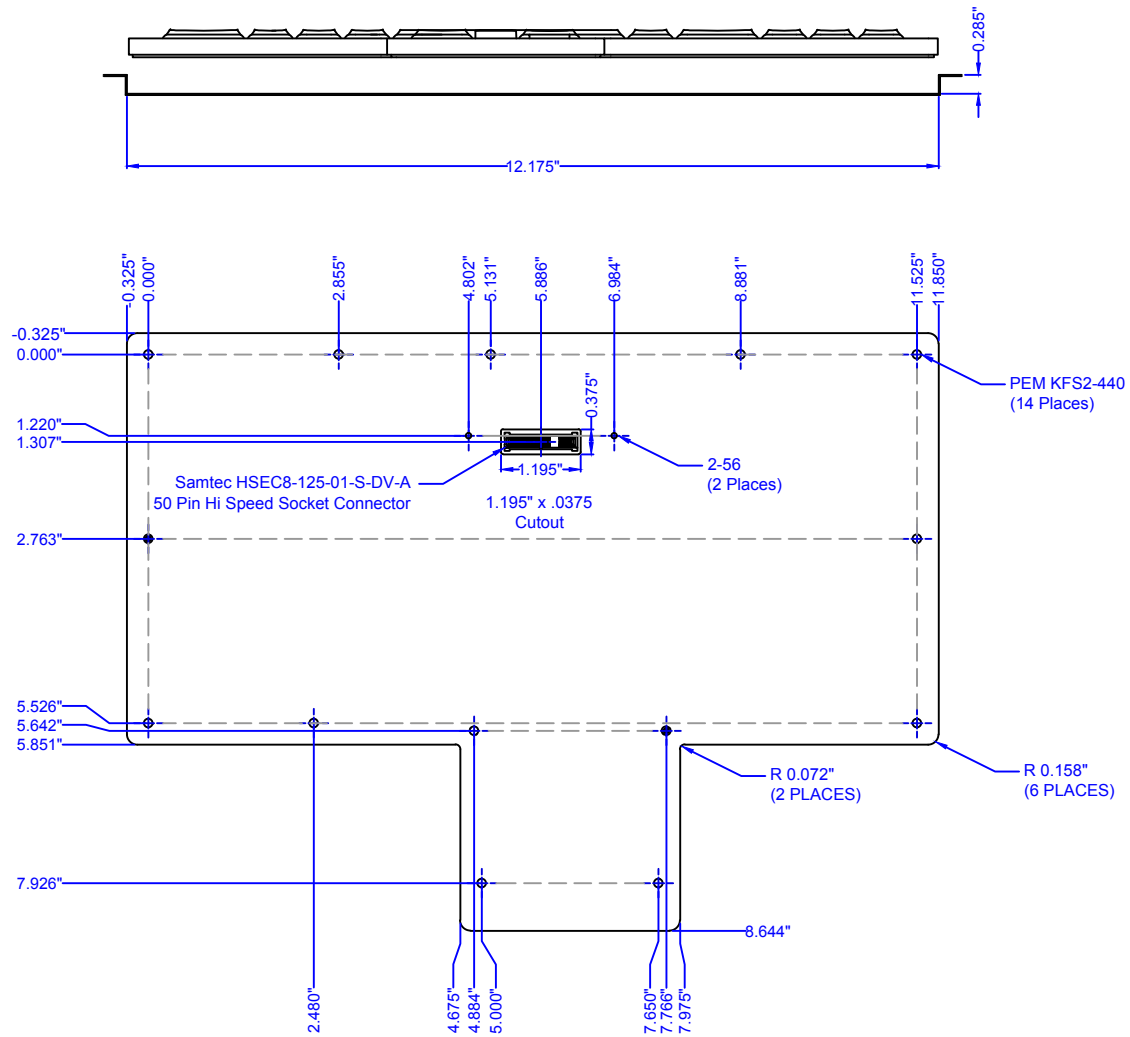
Bottom View
